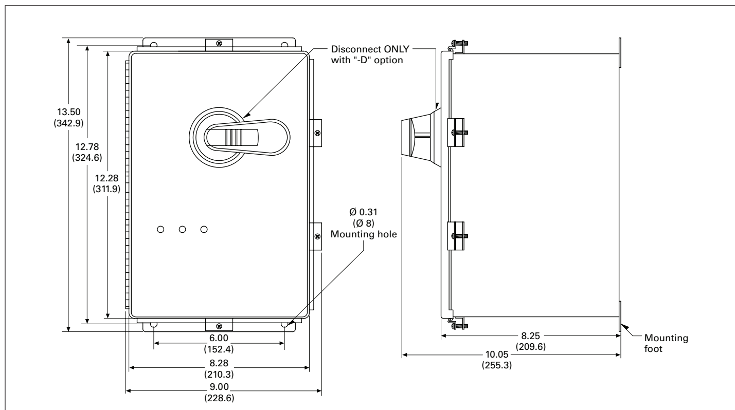
Figure 6. Protector series for the integral circuit breaker (-C) and circuit breaker and external disconnects (-CD) 80, 120 ① , 160, 240 ① and 300 kA models
