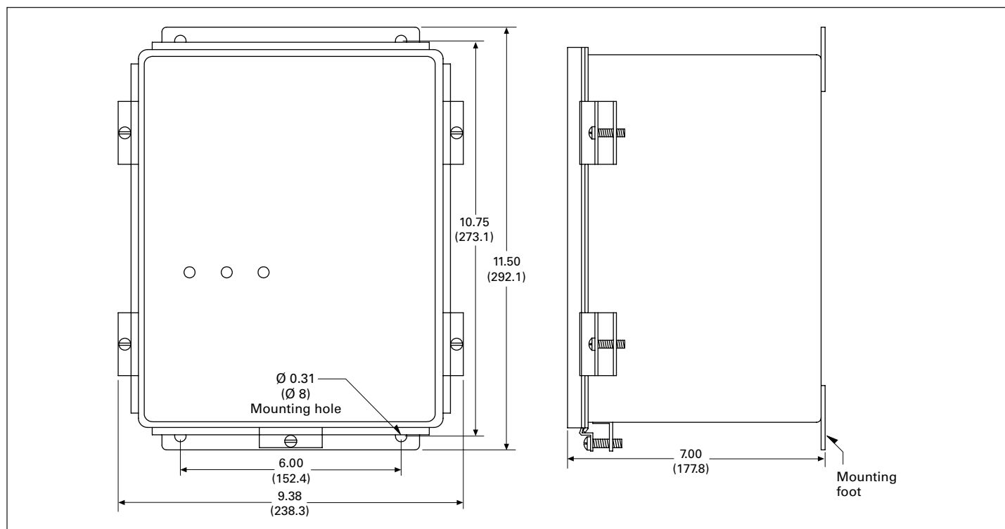
Figure 5. Protector series for PTE/PTX240 low-voltage models, PTE/PTX300 all models and PTE/PTX 400, all models
