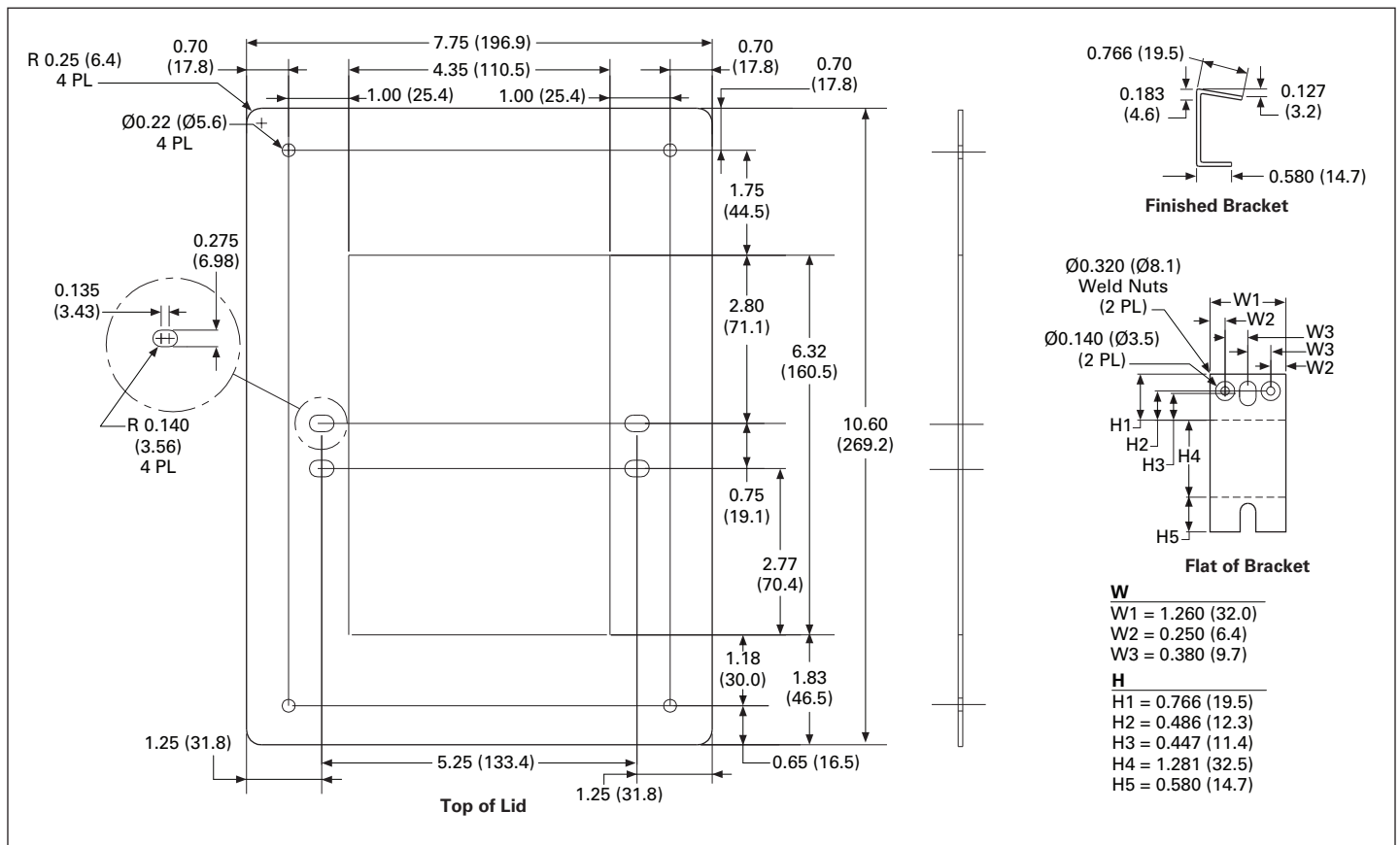
Figure 8. FLUSHMNTPLATE3A PTE/X units 40, 65, 80 kA
