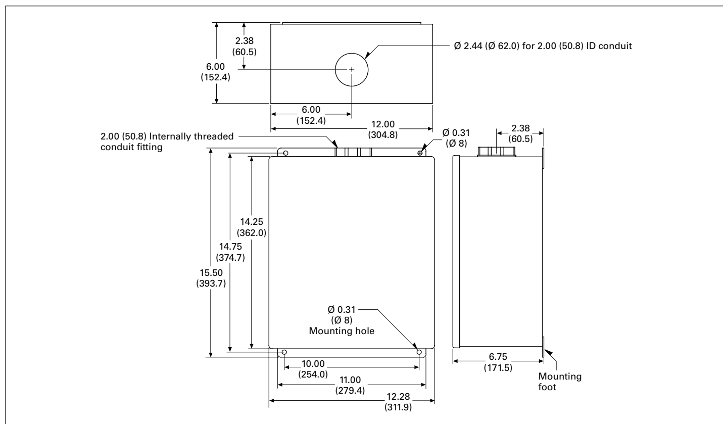
Figure 4. Protector series for PTX240 medium-voltage models only
