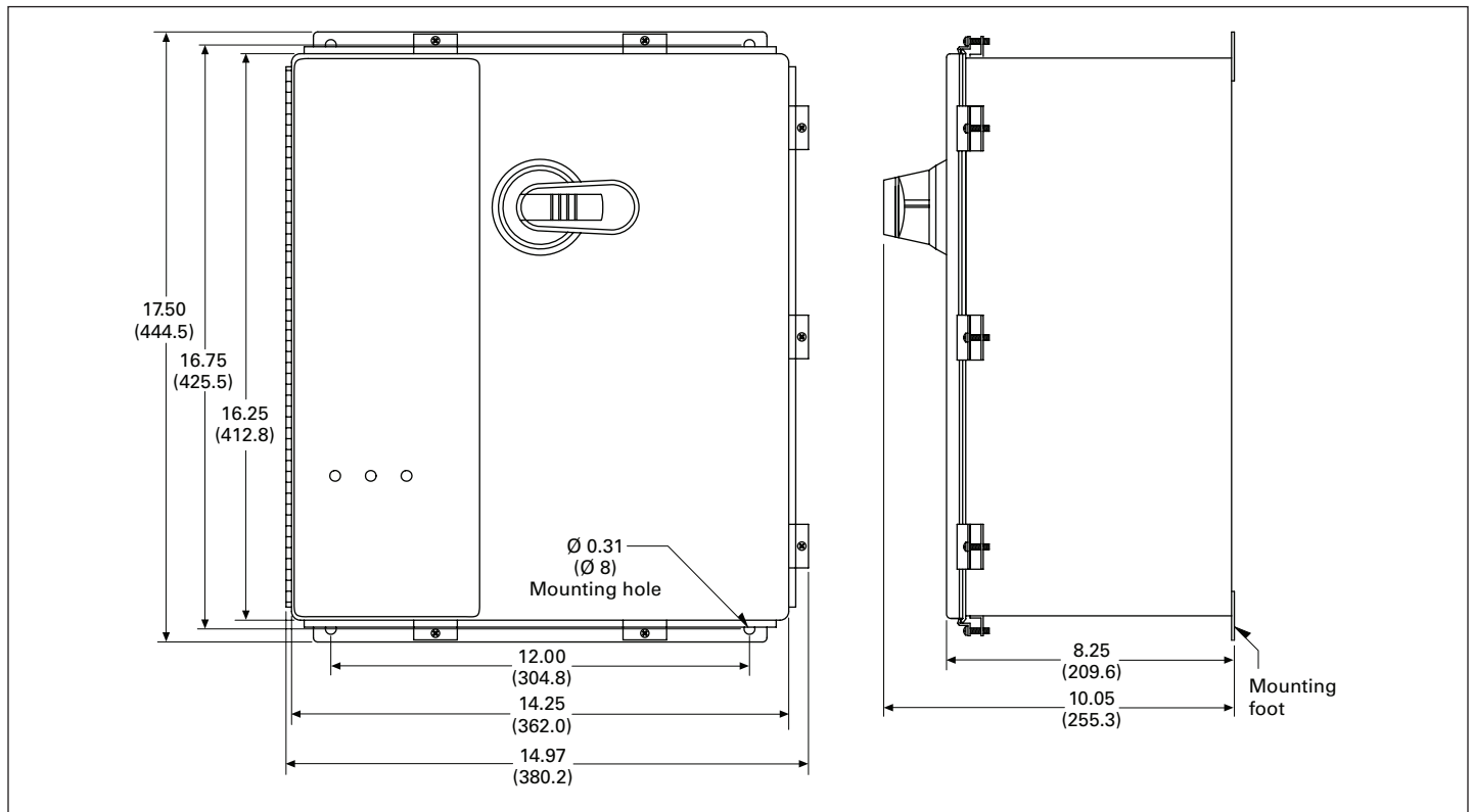
Figure 7. Protector series for integral circuit breaker (-C) and circuit breaker and external disconnect (-CD) 400 kA models
