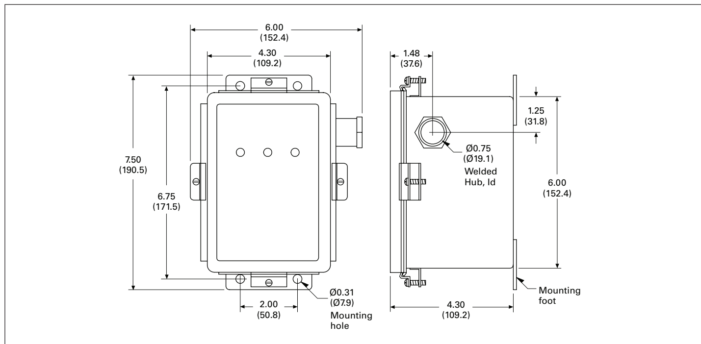
Figure 1. Protector series for PTE048, 065, 080 Models 1P101, 1S101, 3Y101, 3D101 and PTX048, 065, 080 all models
