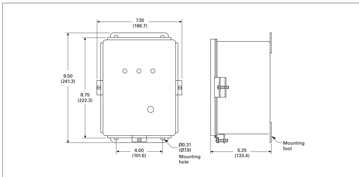
Figure 2. Protector series for PTE048, 065, 080 models 1P201, 3Y201, 3Y300, NN201, NN400, NN501, PTE/PTX 120 low-voltage models, and PTE/PTX 160 all models
