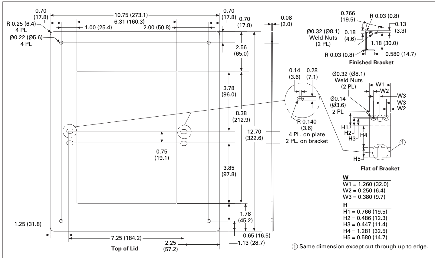
Figure 9. FLUSHMNTPLATE8 PTE/X units 120 and 160 kA
