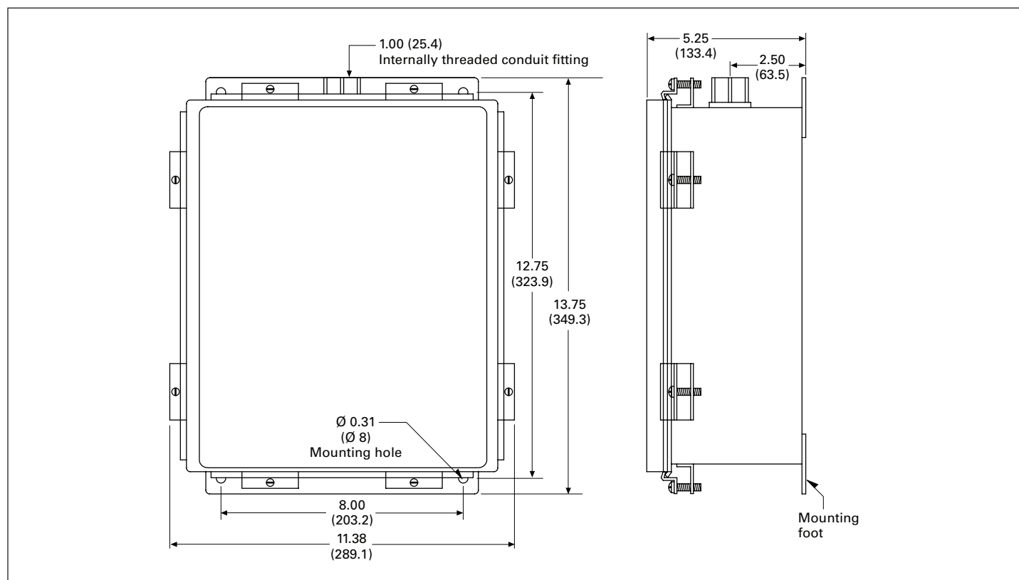
Figure 3. Protector series for PTX120 medium-voltage models only
